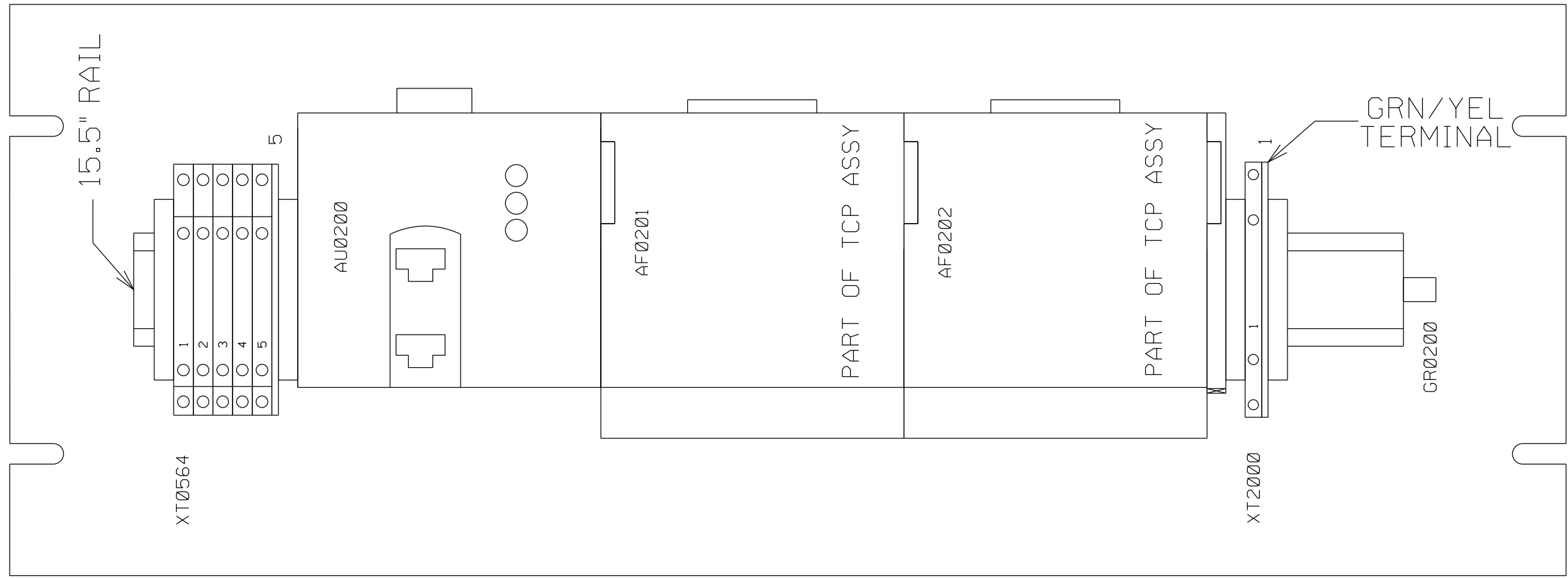
BACK VIEW WITH FLEX I/O INSTALLED TYP. FOR XT0564
